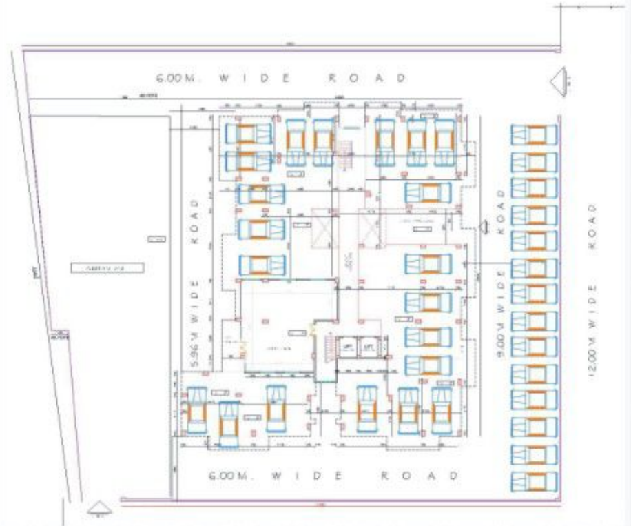
Stilt Floor Plan
